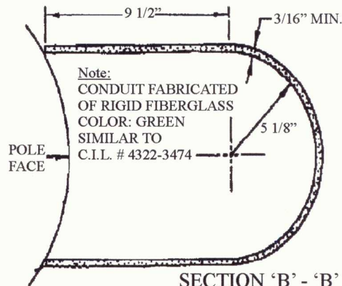
SECTION 'B' - 'B' SCALE : 3/8" = 1"
