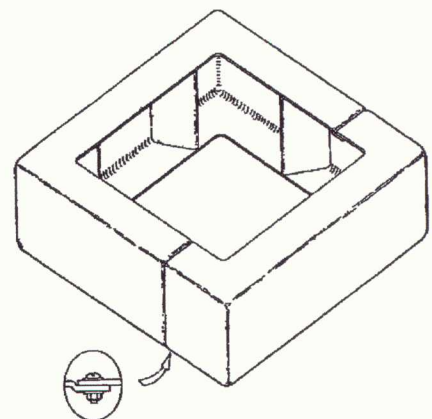
LIP JOINT DETAIL
